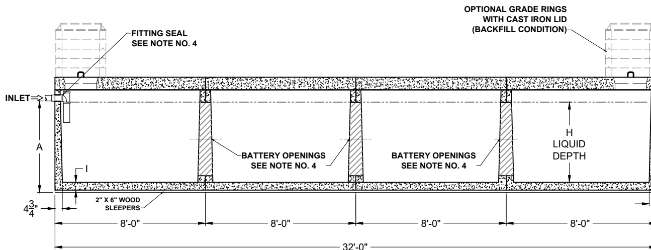
SECTION THRU "A-A"
